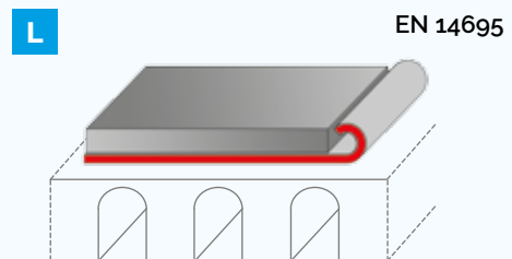
Waterproofing under bituminous conglomerate
